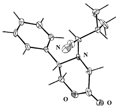
Fig. 1 X-Ray structure of major adduct 3a .
