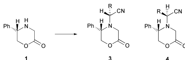
Scheme 2 Reagents and conditions: CuCN, HCl (anhyd.), Na 2 SO 4 (anhyd.), RCHO, THF.
