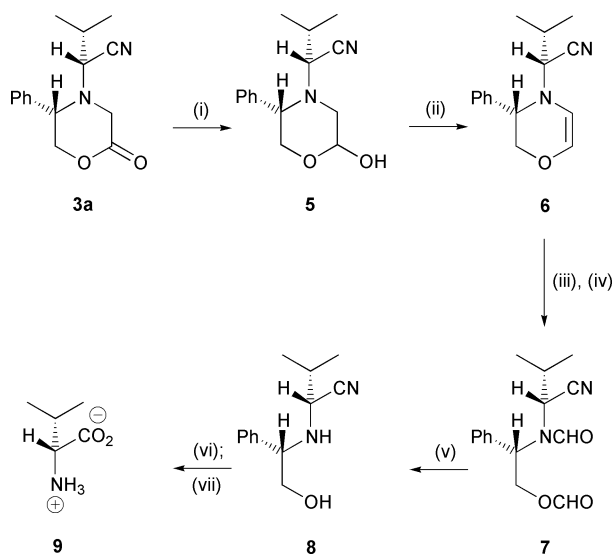
Scheme 3 Reagents and conditions: (i) DIBAL-H, THF, -78\text{ }^{\circ}\text{C} ; (ii) \text{Ac}_2\text{O} , \text{BF}_3\cdot\text{OEt}_2 , MeCN, rt; (iii) MCPBA, DCM; (iv) \text{H}_2\text{IO}_6 ; (v) EtOH, \text{TiCl}_4 , rt; (vi) \text{Pb}(\text{OAc})_4 , MeOH-DCM, 0\text{ }^{\circ}\text{C} ; (vii) conc. HCl.
