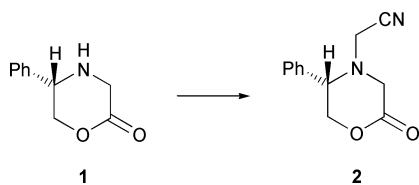
Scheme 1 Reagents and conditions: CuCN, HCl, (CH 2 O) n , THF, rt.
